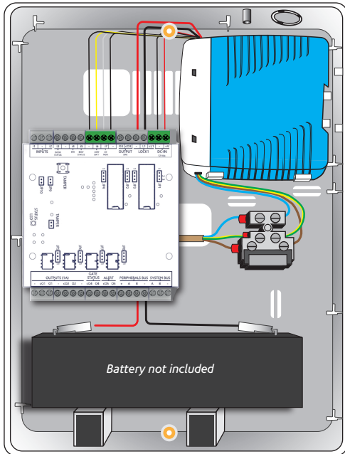
Kit UPS 13.8V/60W - KSI7101260.000
