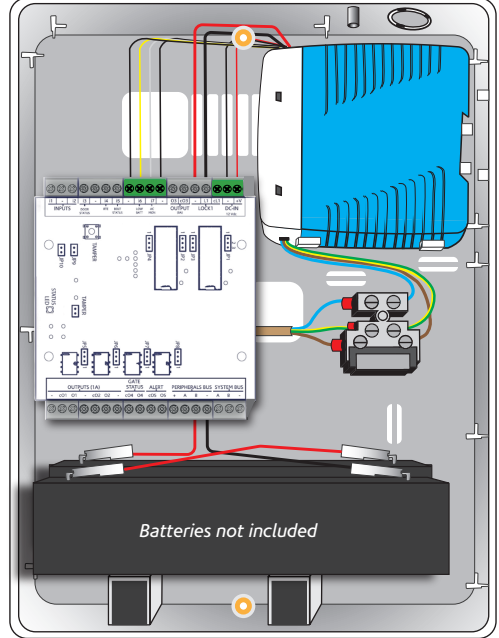
Kit UPS 27.6V/60W - KSI7102460.000
